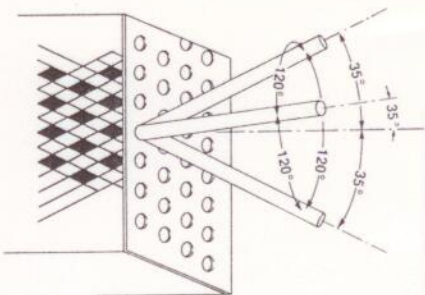
Figure 2 The method of constructing an f.c.c. lattice of the Wigner-Seitz cells as shown in Fig. 1b. A slab of material is covered by a mask consisting of a triangular array of holes. Each hole is drilled through three times, at an angle 35.26^\circ away from normal, and spread out 120^\circ on the azimuth. The resulting cross-section of holes below the surface of the slab, suggested by the cross-hatching shown here, produces a fully 3-d periodic f.c.c. structure, with unit cells as given by Fig. 1b. The drilling can be done by a real drill bit for microwave work, or by reactive ion etching to create an f.c.c. structure at optical wavelengths.
